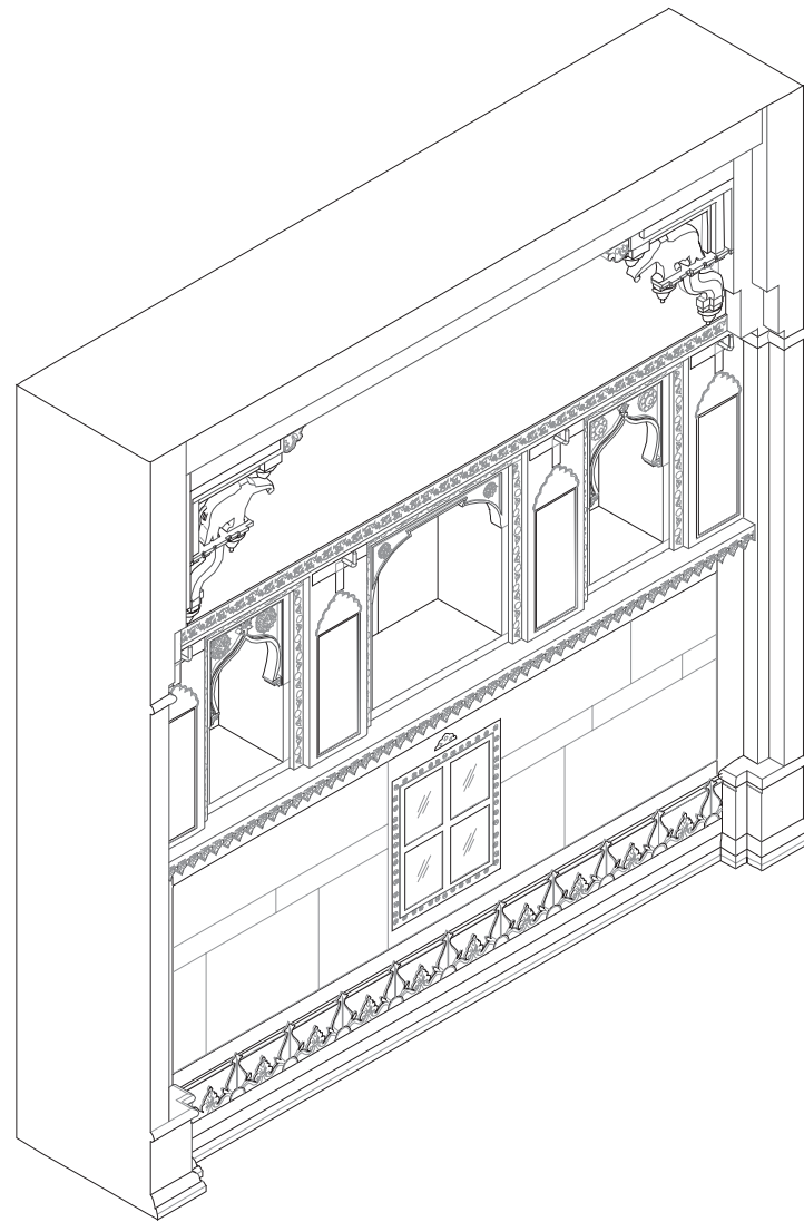
Isometric View
