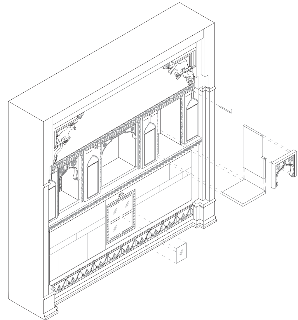
Exploded Isometric View
