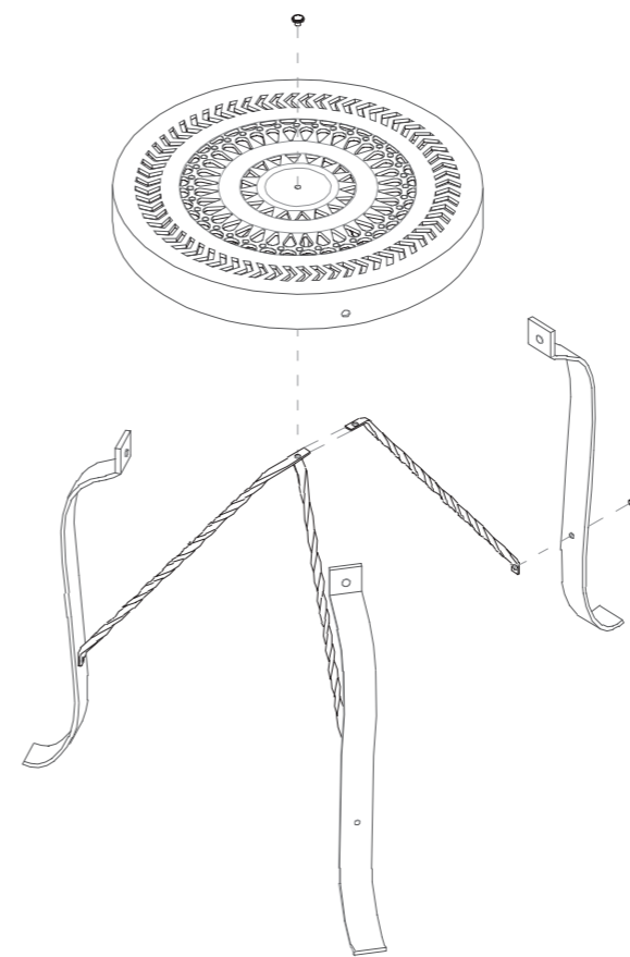
Exploded Isometric view
