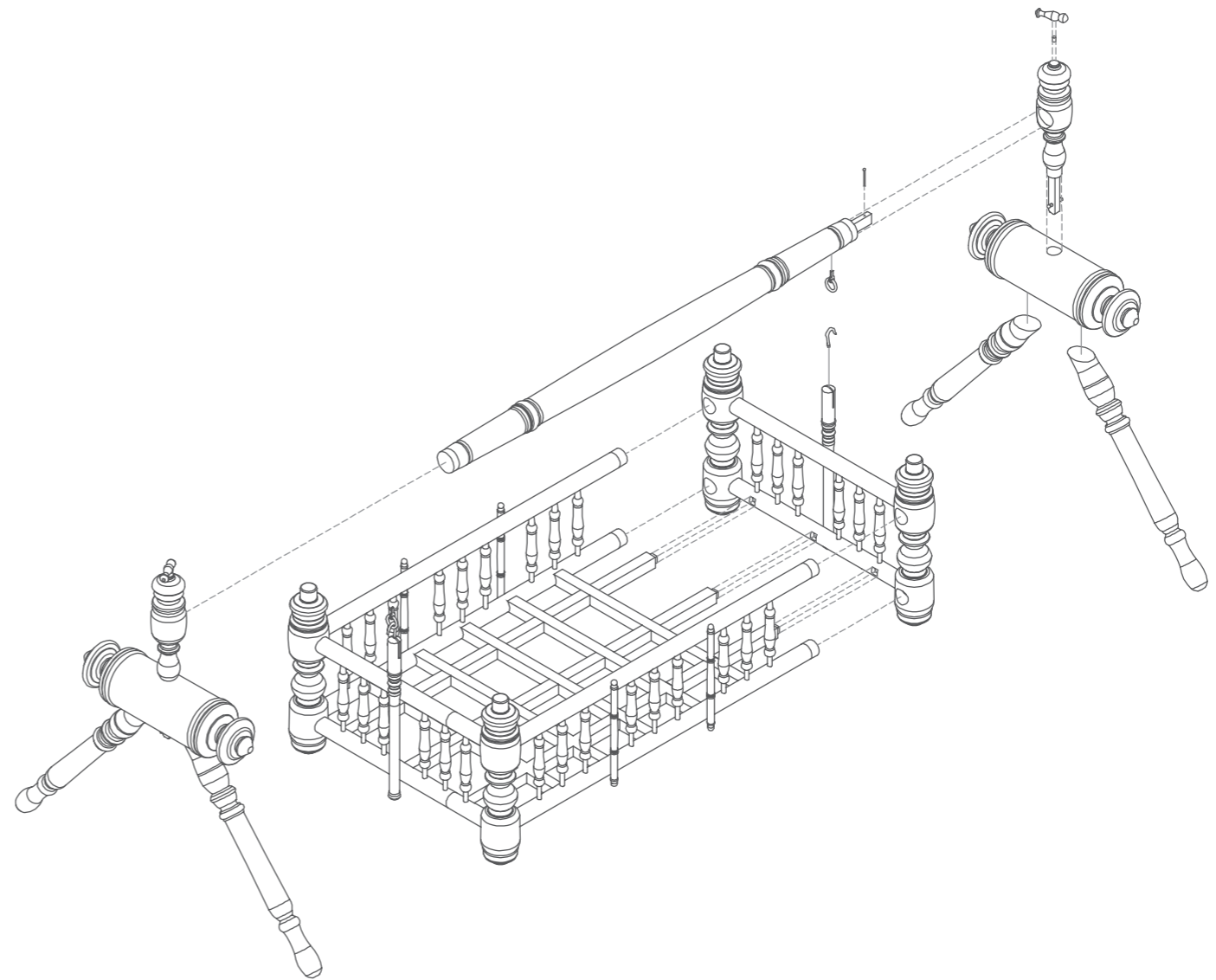
Exploded view
