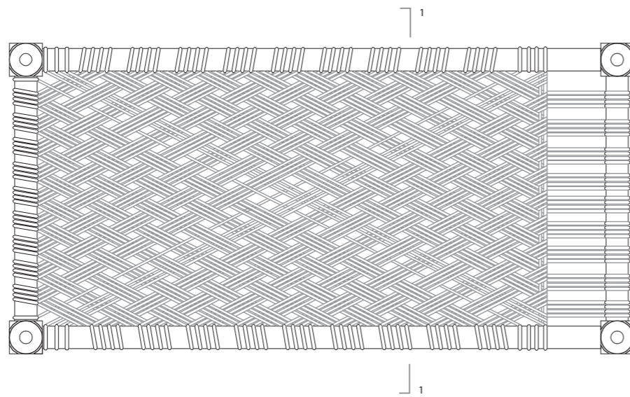
Plan (Top view)
