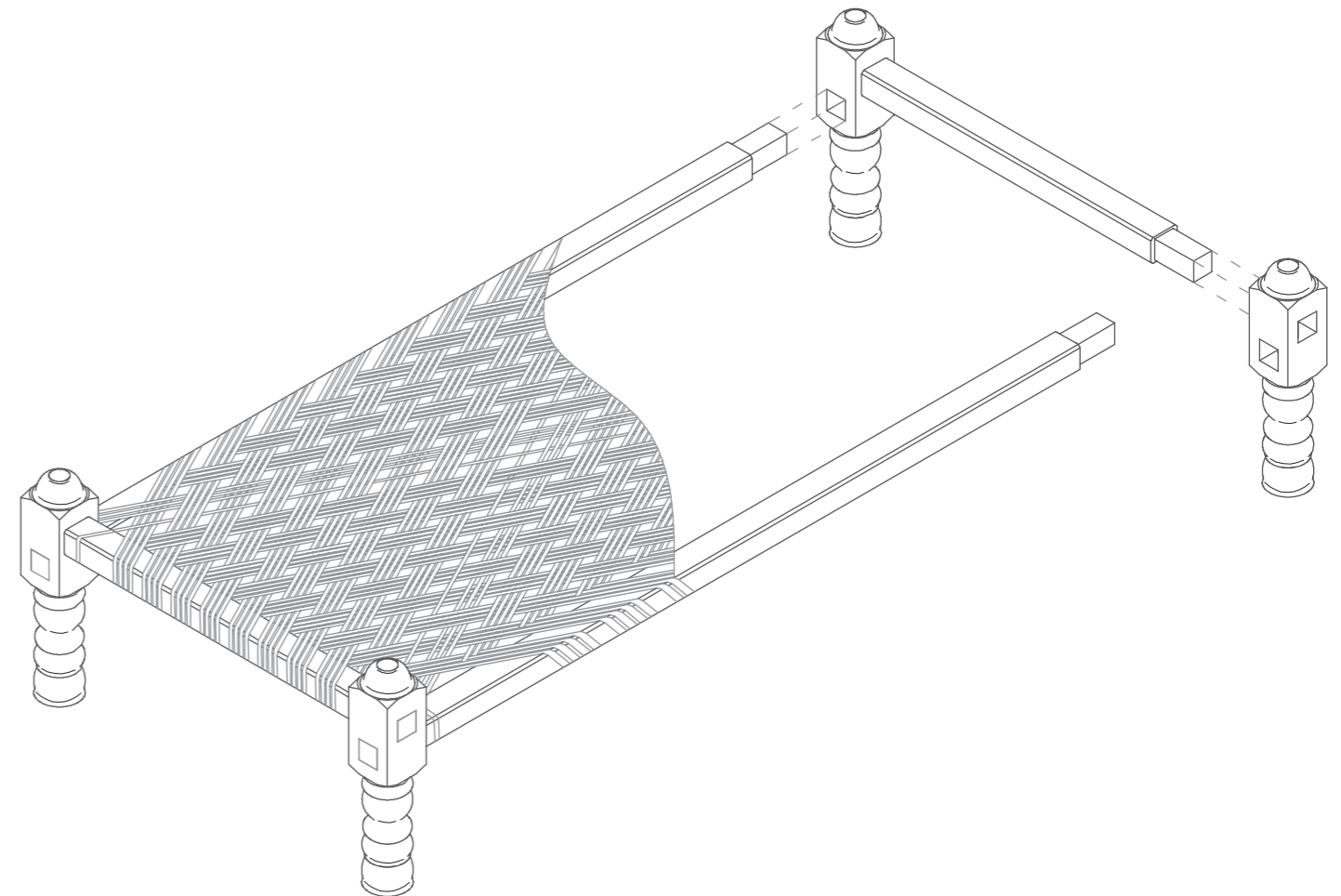
Exploded view
